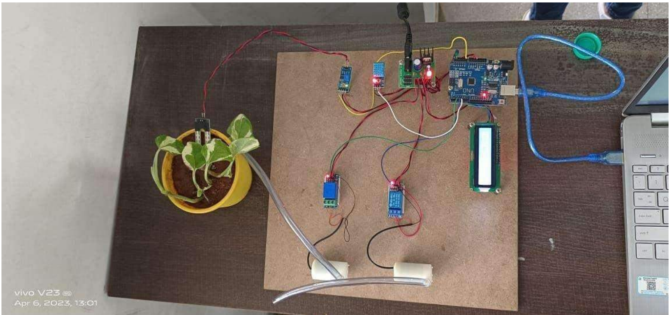
Innovation 5: Automatic indoor Plant Health Management System using Arduino
