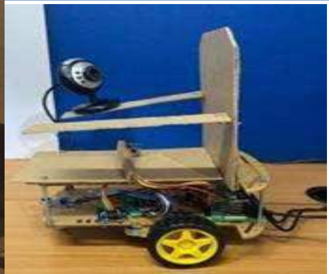
Innovation 2: Ocular based Wheelchair Actuator System for Amyotrophic lateral Sclerosis impaired patients
